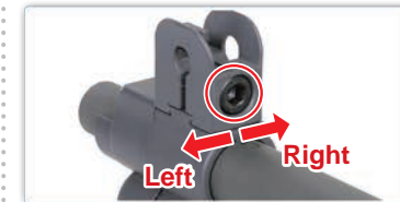
1. Remove the screw 2. Push the front sight to either direction for Windage adjustment.
