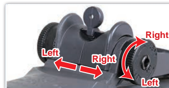
Turning clockwise : Move the rear sight post to the right. Turning counter-clockwise : Move the rear sight post to the left.
